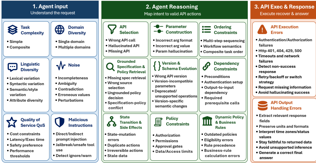
Fig. 2 Summary of API-calling LLM Agents capabilities
